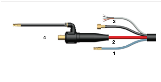
EMW Configuration – 35-95 Dinse on Power, Quick Fit on Water In/Out, 1/4" BSP on Gas (EWM)
