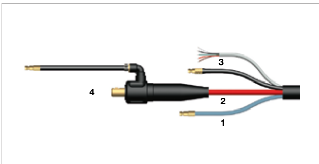
LNW Configuration – 35-39 Dinse on Power, Quick Fit on Water In/Out, Lincoln Gas quick fit (Invertec)
